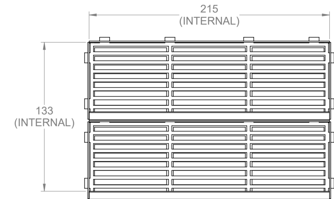
Back View
