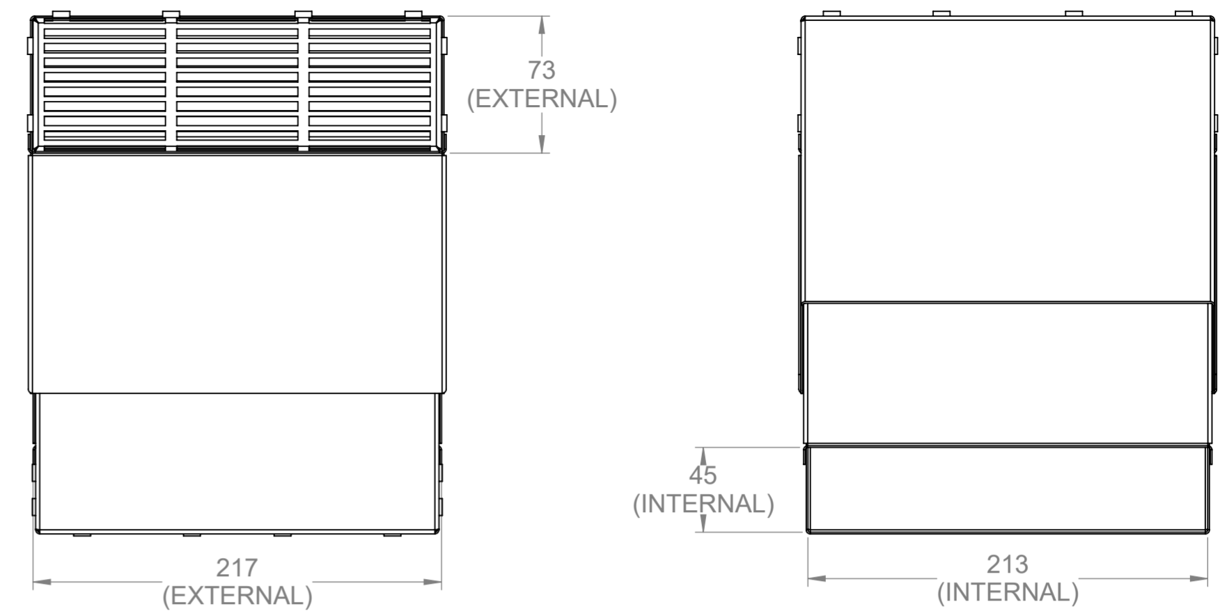
Front View
