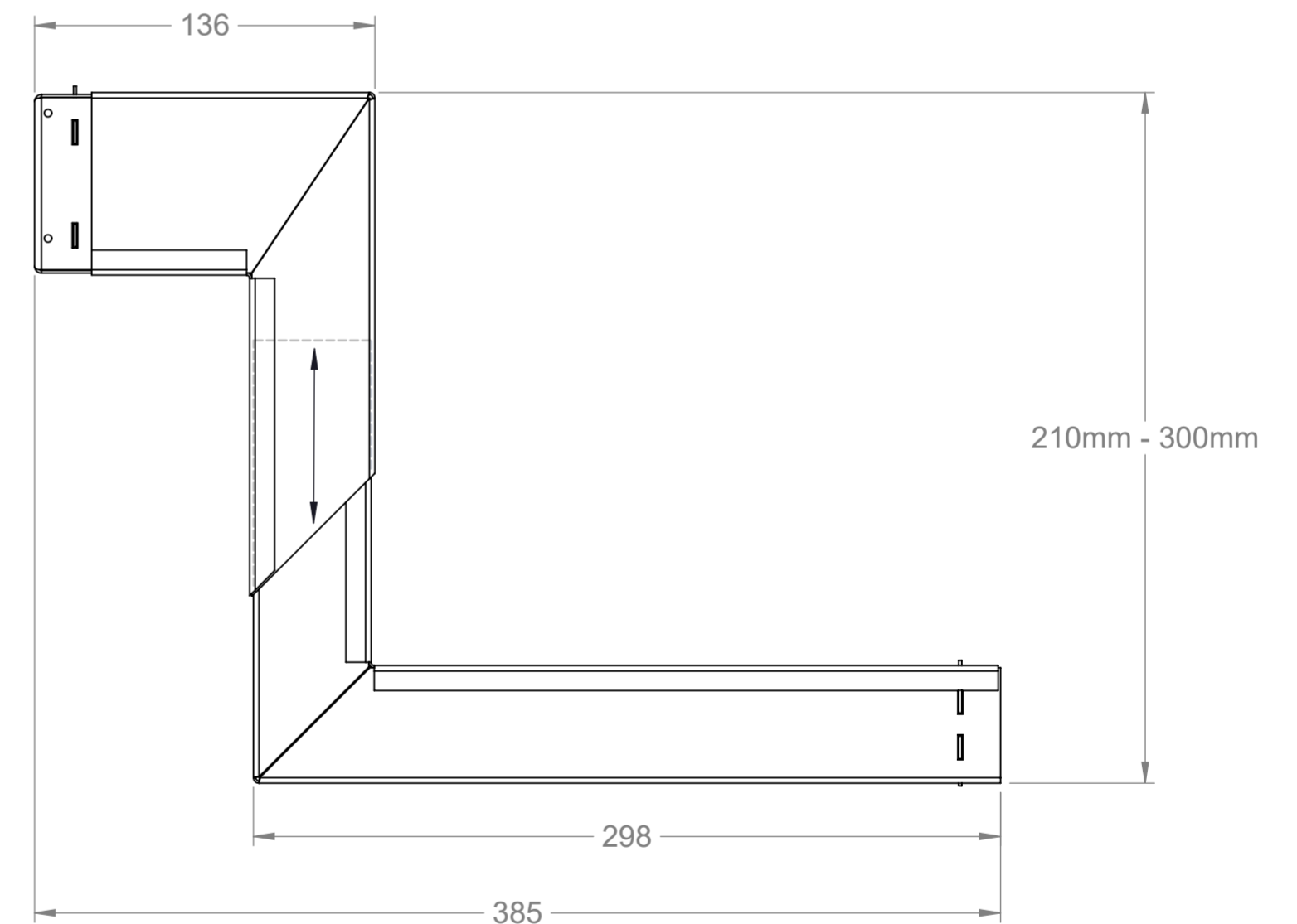
Side View
