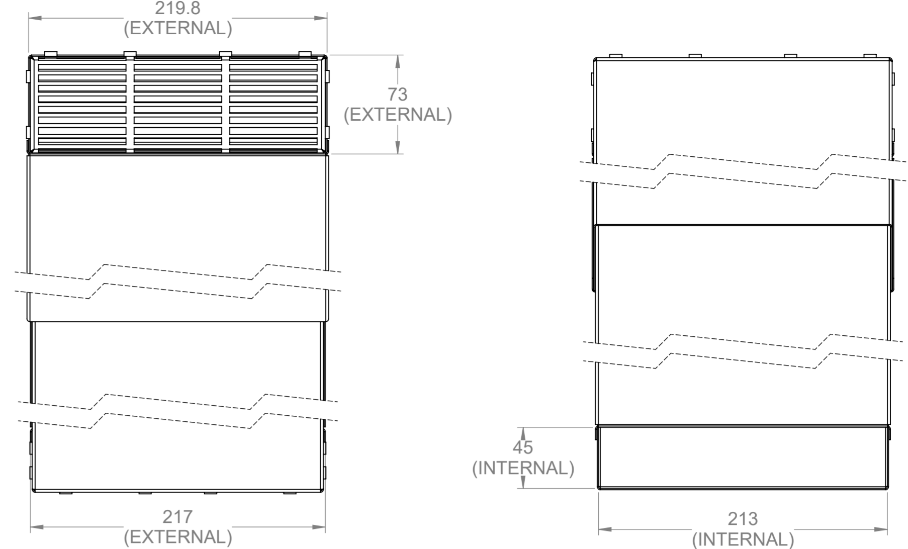
Front View
