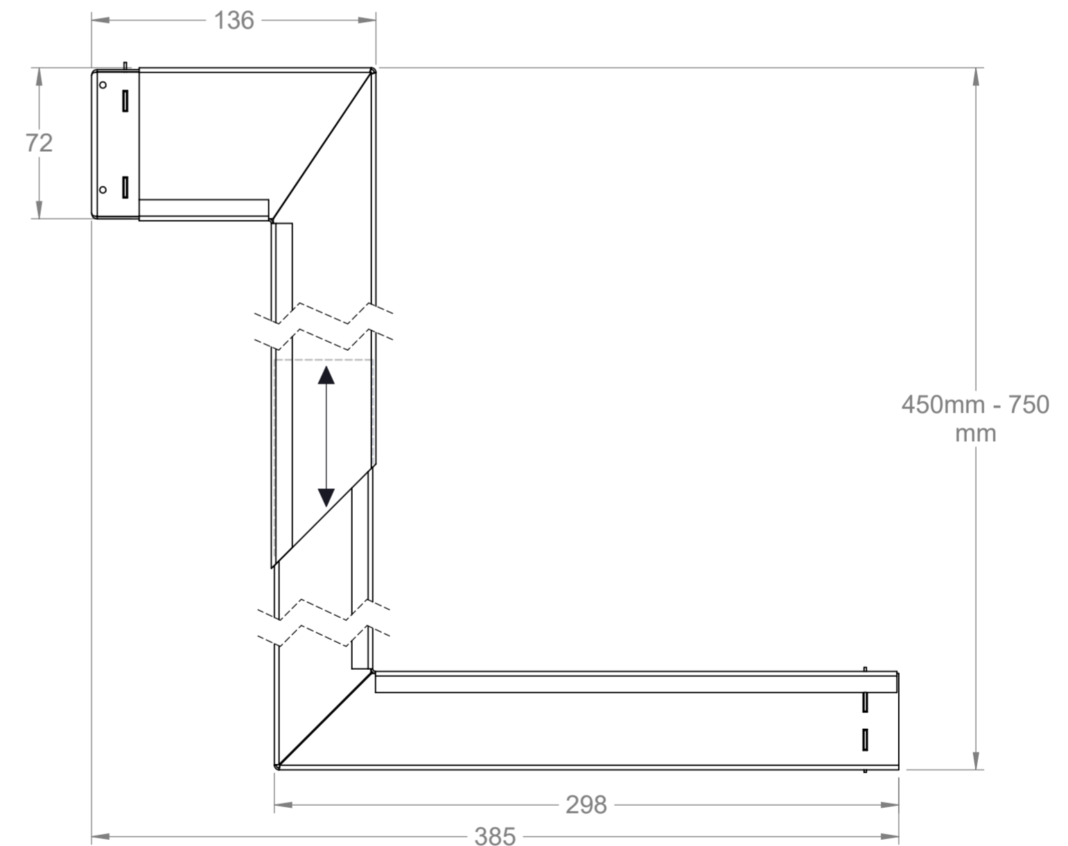
Side View
