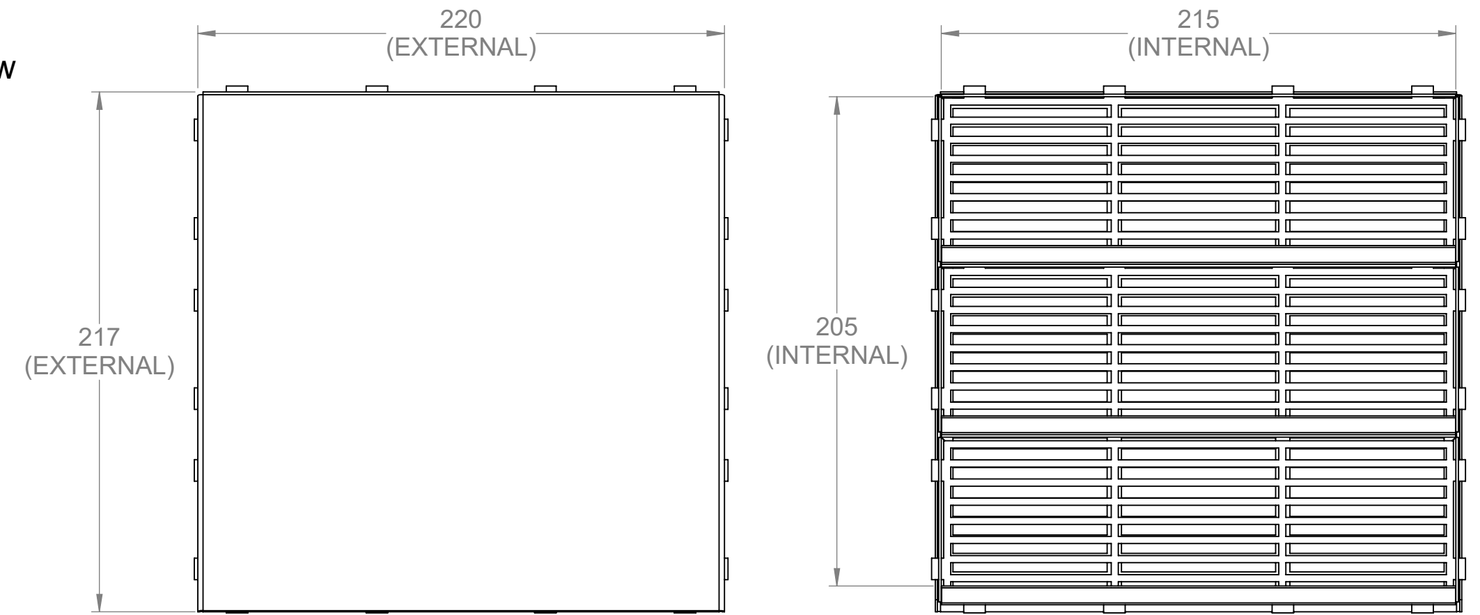
Front View
