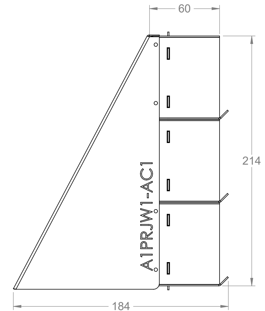
Side View
